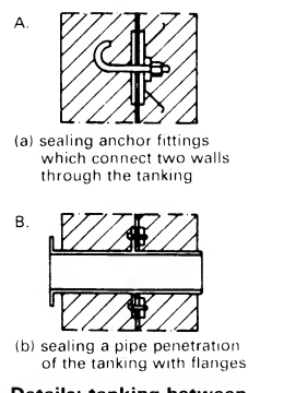
⑨ Details: tanking between two walls
